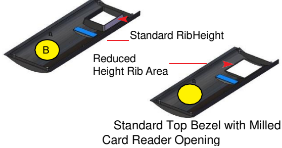
Standard Top Bezel with Card Reader Opening
